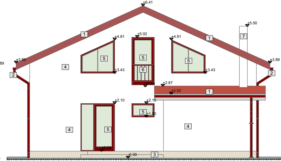
FATADA VEST
